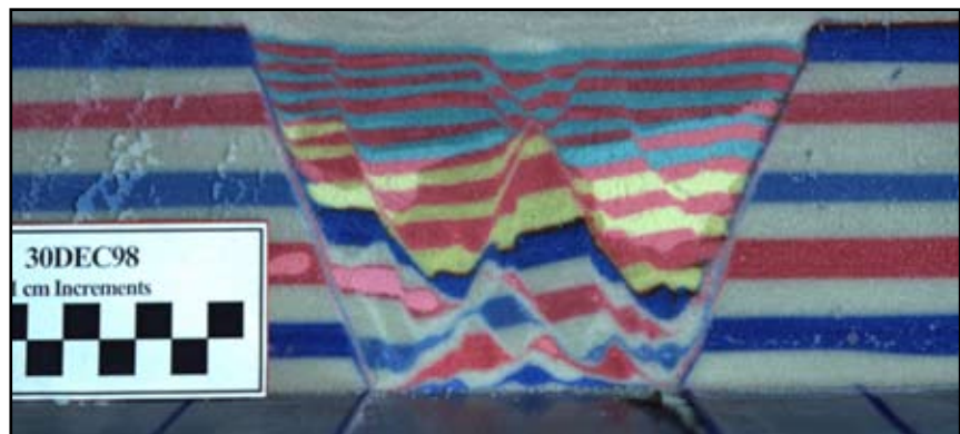
Cross-section of sand model of pull-apart basin showing graben in growth strata (blue and red) above horst earlier growth strata (yellow and red).
