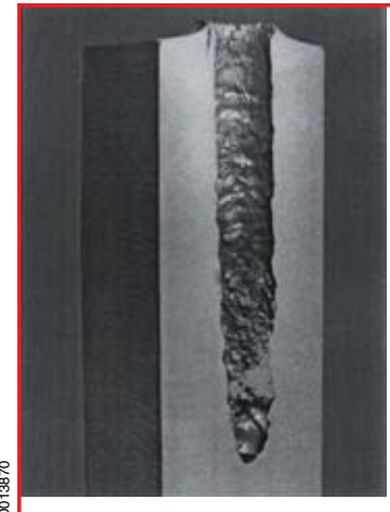
Penetration channel for an L/D 30 tungsten-alloy projectile into an armor steel target
